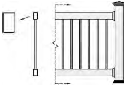
Traditions Series 100 1.3" Square Balusters
