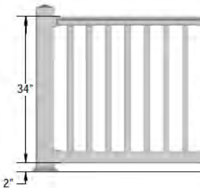
Superior Series 200 1.3" Square Balusters
