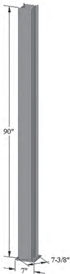
6" Sq. Column Mount
