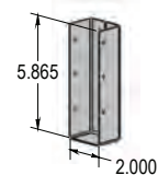
2" x 6" Wall Mount Bracket
