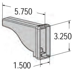
1 1/2" x 3 1/4" Pergola End
