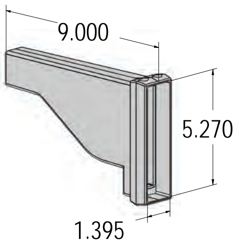
1 3/8" x 5 1/4" Pergola End
