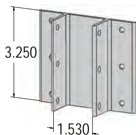
1 1/2" x 3 1/4" Wall Mount Bracket
