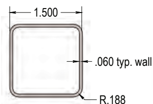
1 1/2" Sq. Shade Cover
