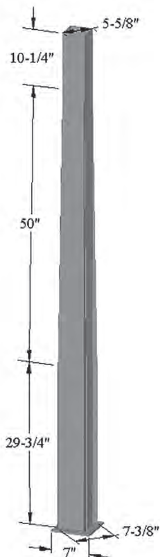
Column Mount
