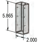
2" x 6" Wall Mount Bracket
