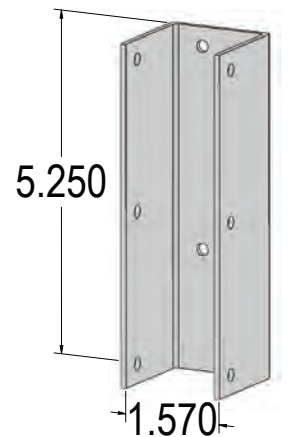
1 3/8" x 5 1/4" Wall Mount Bracket
