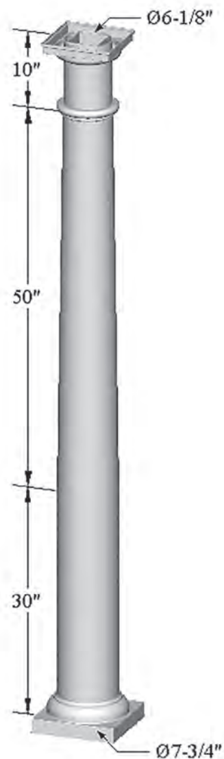
8" Tapered Column
