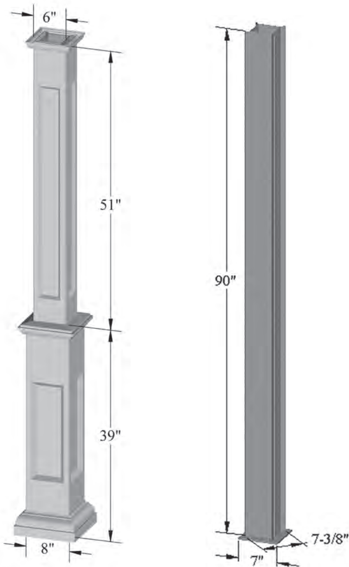
Savannah Column
