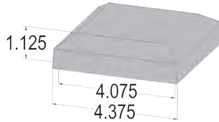
Post Cap
