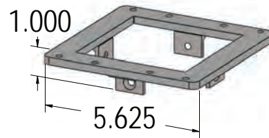
Beam Mount
