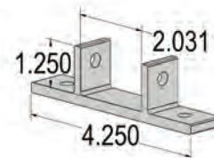
1 1/2" Rafter Bracket
