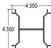
5" Post Insert
