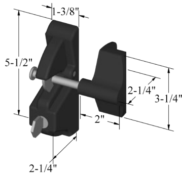
Lockable Latch S2 LLAA
