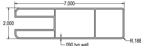
Smooth Rail
