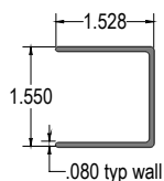
Alum. U-Channel
