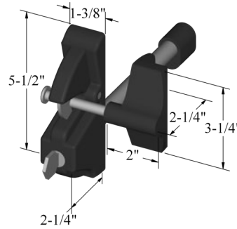
Lockable Latch w/Easy Access Kit LLAAB (Shown) LLDAB-K (Deluxe version)
