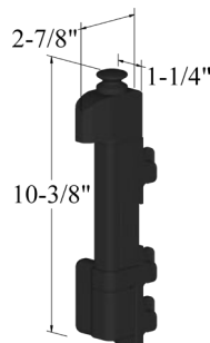
10" MagnaLatch MLVPS2WTBGA (White Only)
