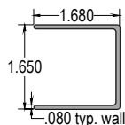
Privacy U-Channel
