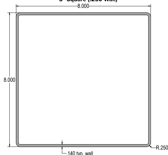
8" Square (.140 Wall)
