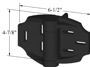
Heavy Duty Multi-Adjust Hinge Self-Closing (Recommended for all 5" or larger posts.) TCHDMA1
