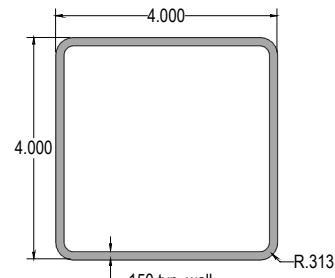
4" Square (.150 Wall)
