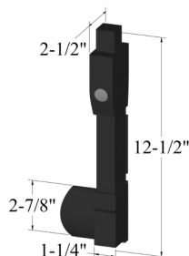
10" MagnaLatch ML3VPKA
