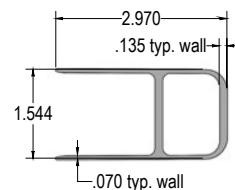
Heavy A-Channel
