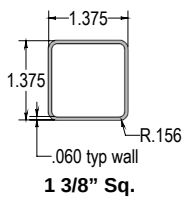
1 3/8" Sq.
