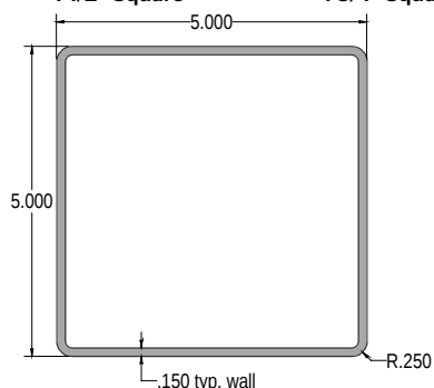
5" Square (.150 Wall)
