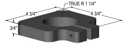
5" Pipe Clamp (2 1/2" Pipe)
