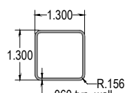
1.3" Square
