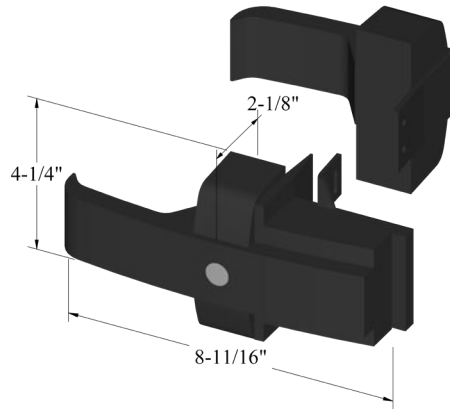
Magnetic Lockable Latch LLMKA
