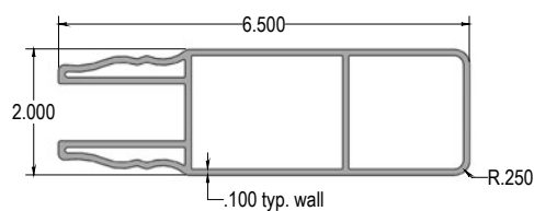
2" x 6 1/2" Deco Rail
