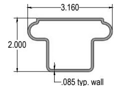
200 Series Top Rail
