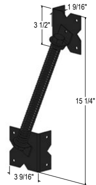
Commercial Spring Set
