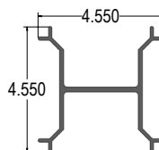
5" Post Insert
