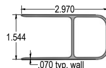
Light A-Channel
