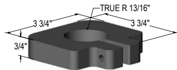
4" Pipe Clamp (1 5/8" Pipe)
