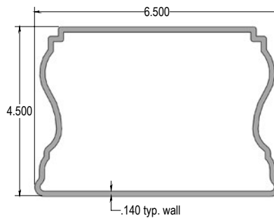
7000 Series Bottom Rail
