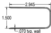
Yard U-Channel
