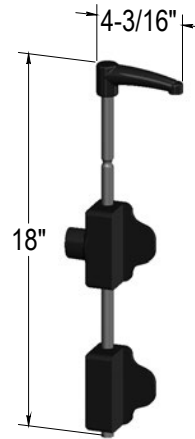
18" Lockable Drop Pin LB218BX-KSA
