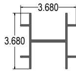
4" Post Insert
