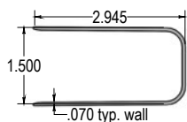
Yard Alum. U-Channel
