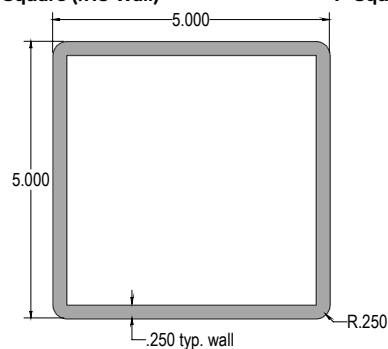
5" Square (.250 Wall)
