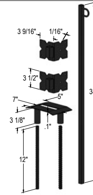
Commercial Drop Pin Kit
