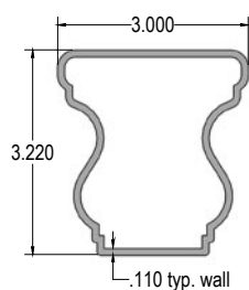
Newport Rail
