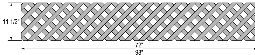
Lattice
