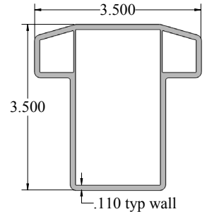
Beveled T-Rail
