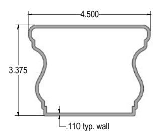
5000 Series Top/Bottom Rail
