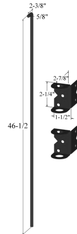
46" Residential Drop Pin Kit
