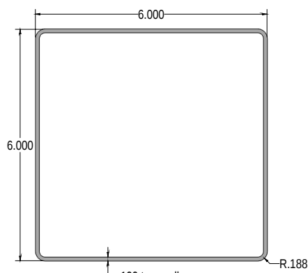
6" Square (.100 Wall)
