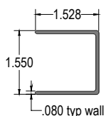
1 3/4" Square Rail Channel
