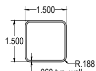
1 1/2" Square
