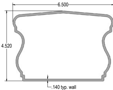
7000 Series Top Rail
