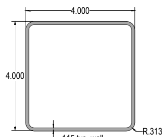
4" Square (.115 Wall)
