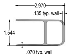
Heavy Alum. A-Channel
