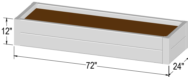
2' x 6' Raised Bed (12" High)
