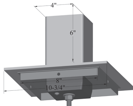
Beam Mount
