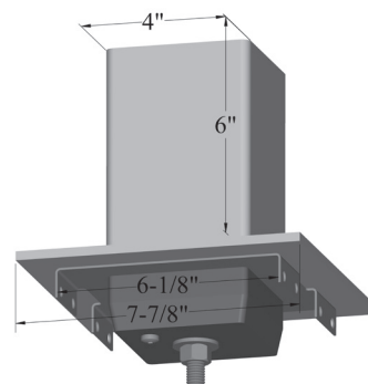
Beam Mount
