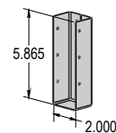
2" x 8" Wall Mount Bracket
