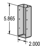
2" x 6" Wall Mount Bracket
