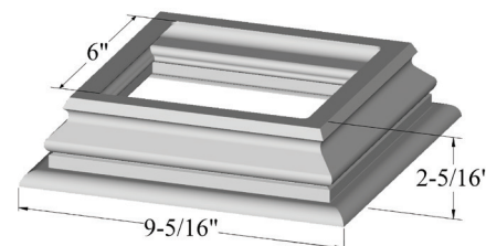
6" Federation Trim
