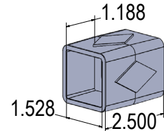
1 1/2" Sq. Shade Cover Coupler
