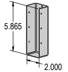
2" x 6" Wall Mount Bracket
