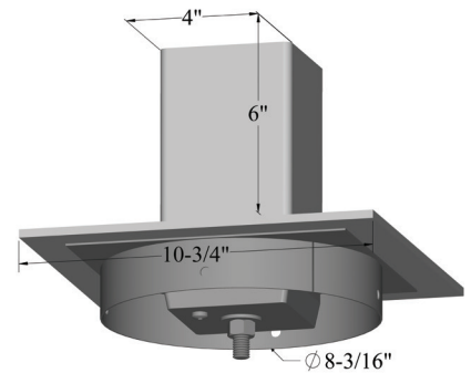
Beam Mount
