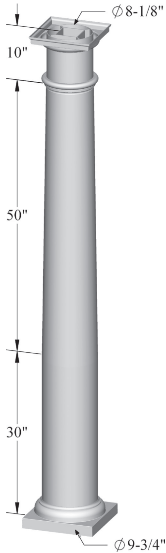
10" Tapered Column
