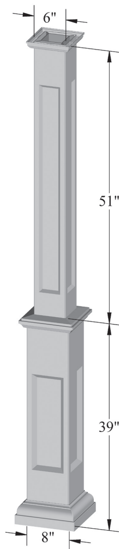
Savannah Column
